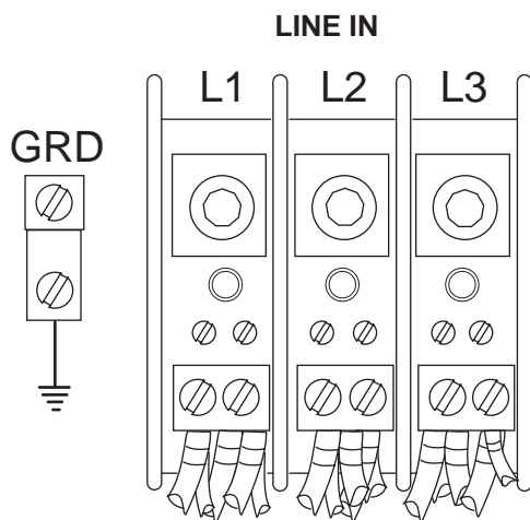
Main Terminal Block Inside the Top-mounted Control Cabinet.
