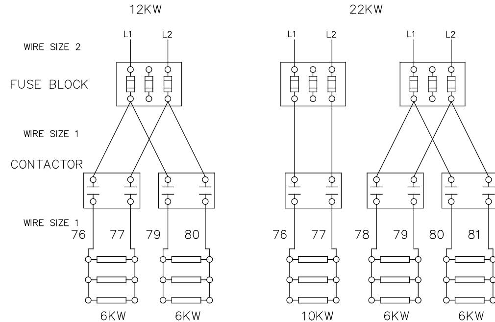
1 PHASE CONNECTION
