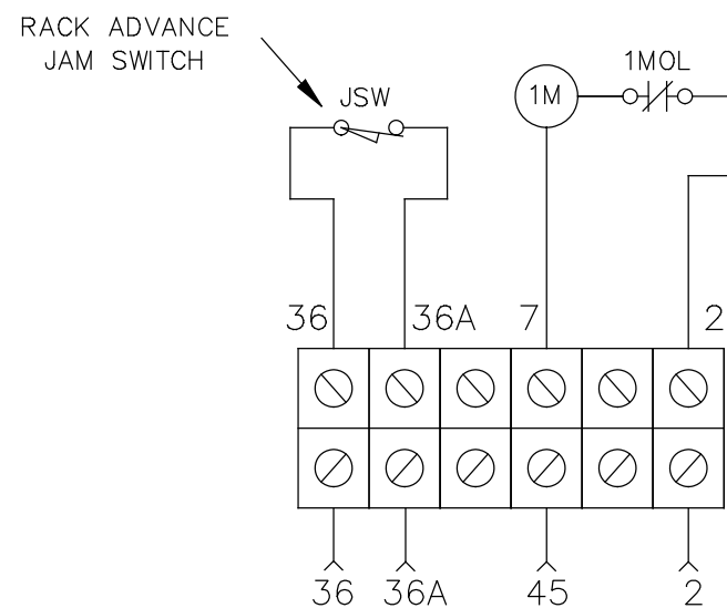
DIGITAL DISPLAY RACK MACHINE MRA WIRING DIAGRAM
