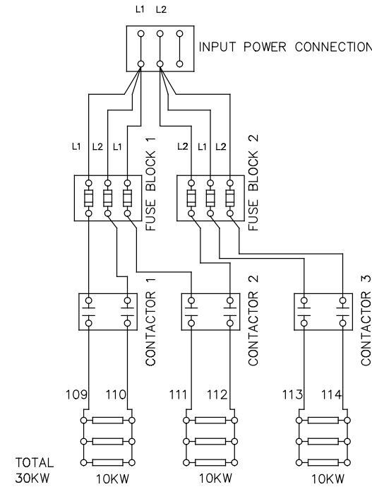
1 PHASE CONNECTION
