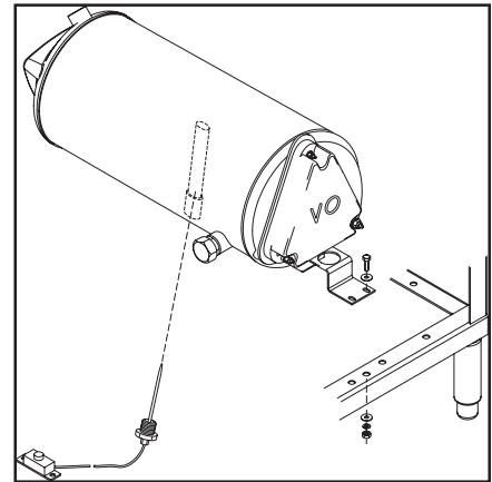
Figure 13- Booster Thermostat Location
