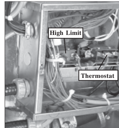
Figure 12- Tank Heat Thermostats
