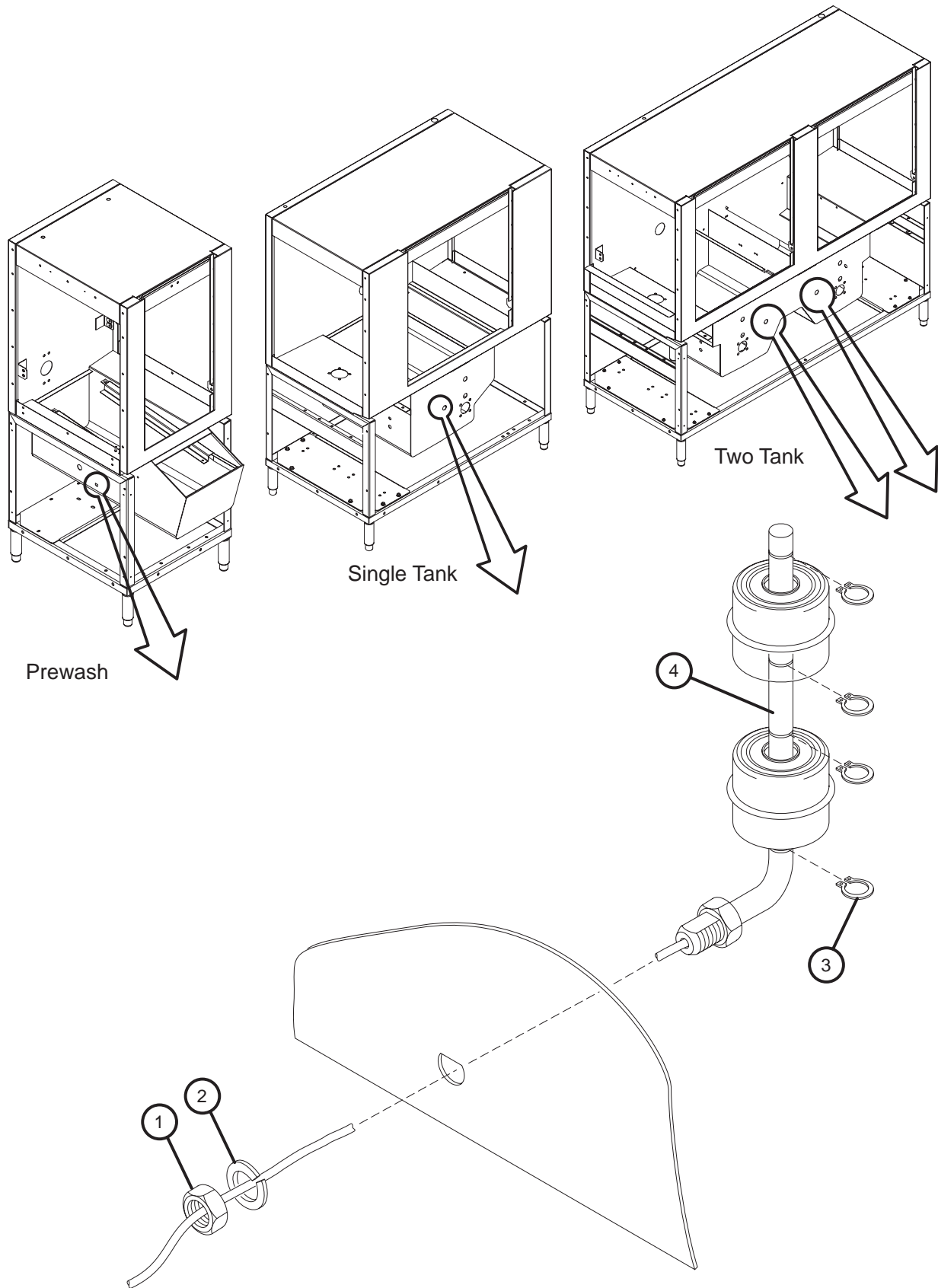
Figure 29- Float Switch
