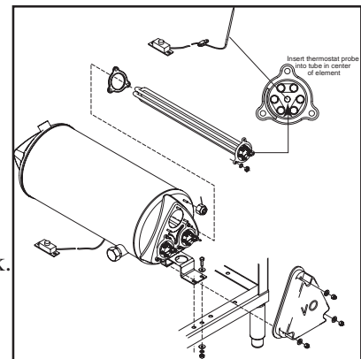
Figure 14- Booster High Limit Thermostat
