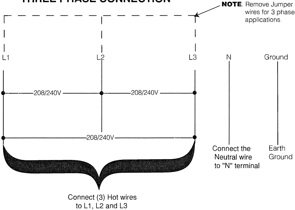
Figure 2 Wiring Connections
