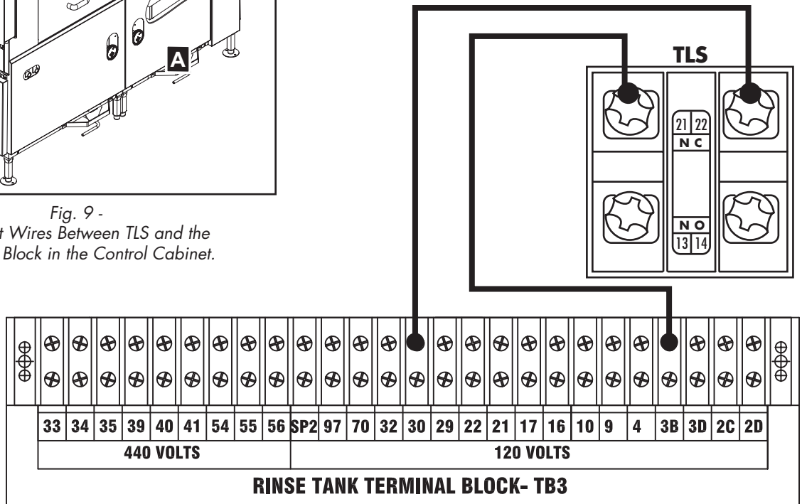
Fig. 10 - Connect Wires between the TLS and the Rinse Tank Terminal Block.
