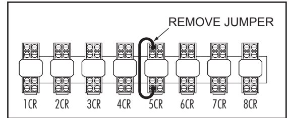
Fig. 8 - Remove Jumper from 5CR relay located in the remote control cabinet.
