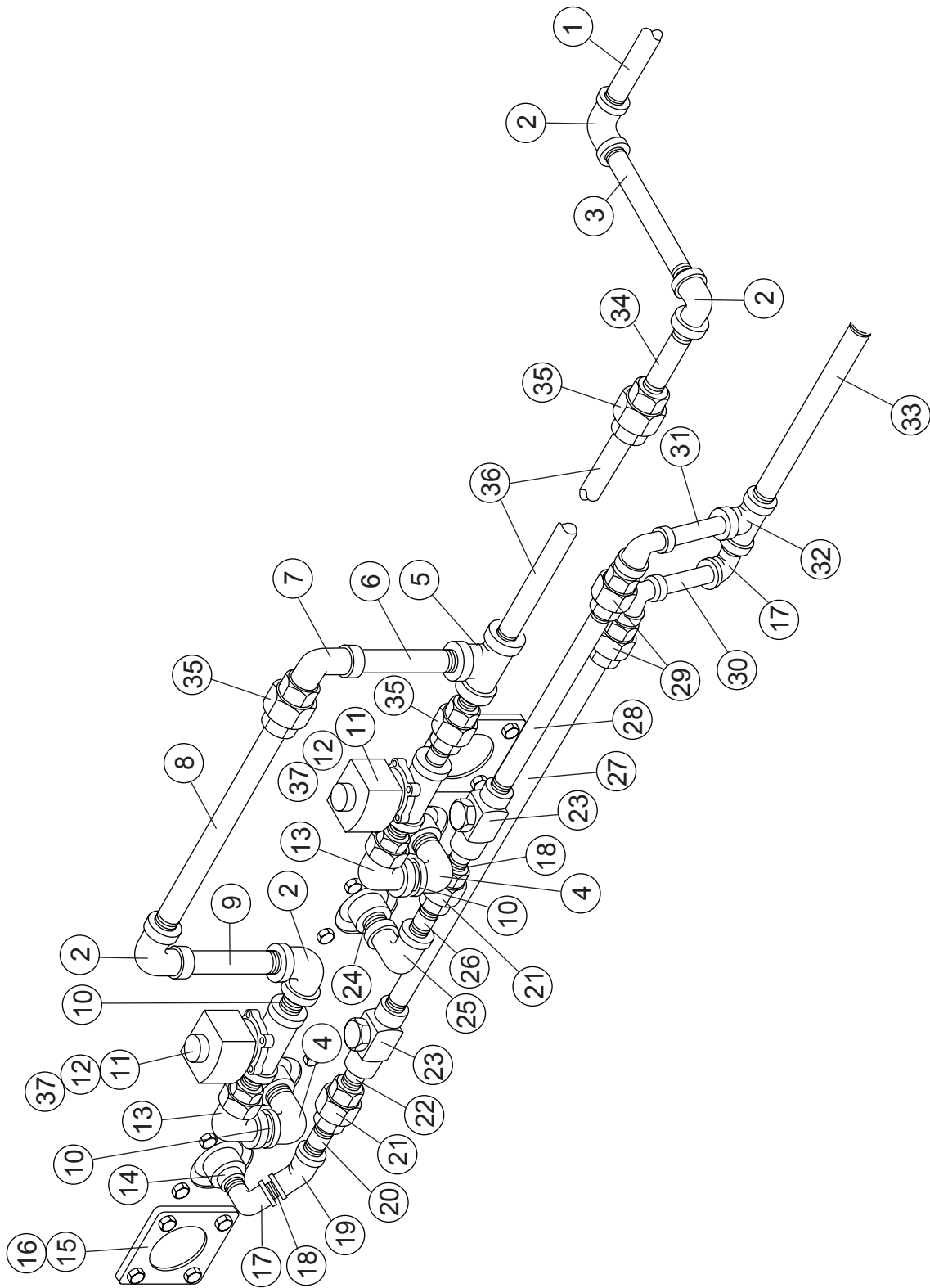
Figure 6.11 - Tank steam piping with booster (L-R machine shown)
