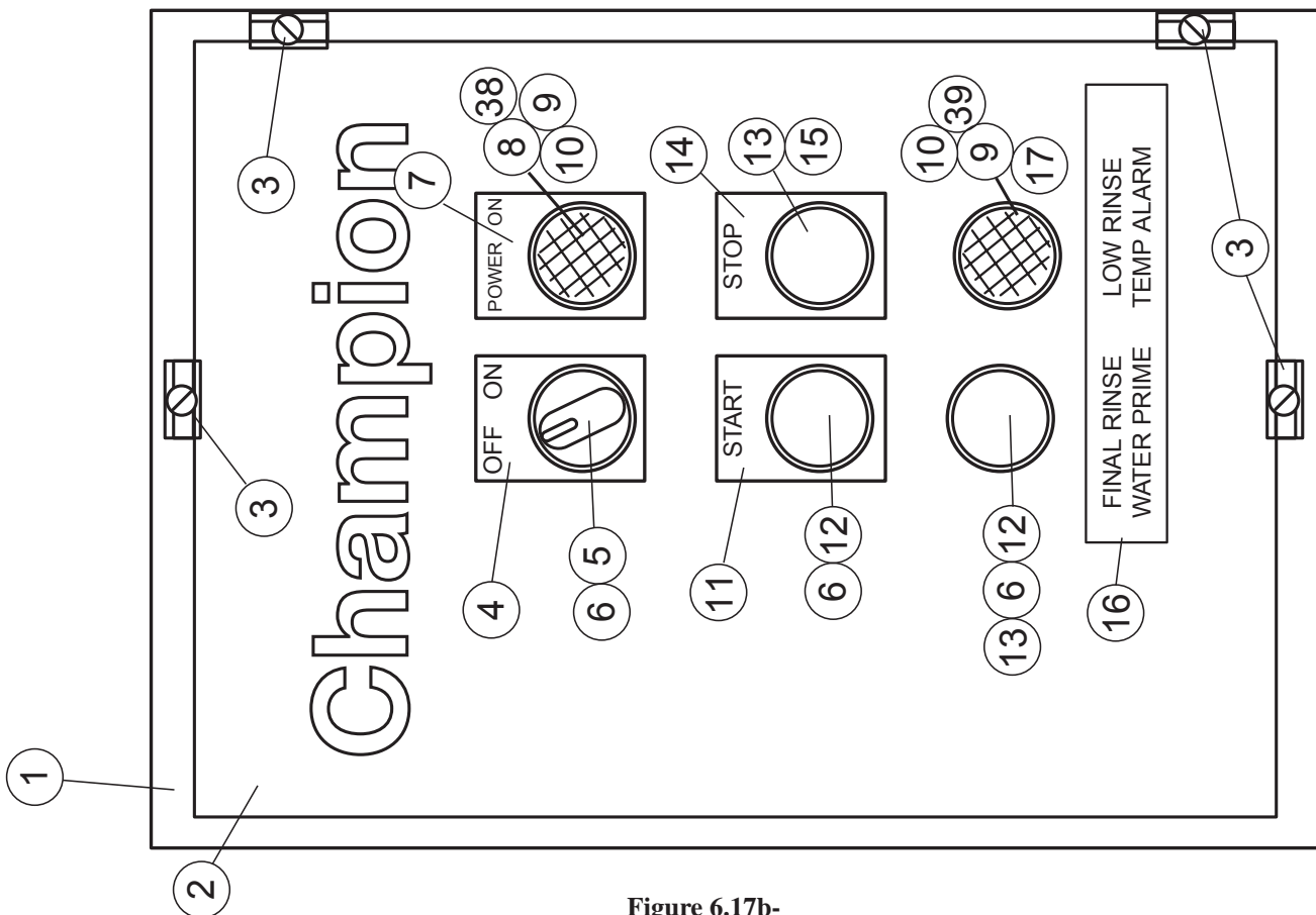
Figure 6.17b- Steam or Electric Remote Control Cabinet (For Machines Beginning with S/N J1080 and Above)
