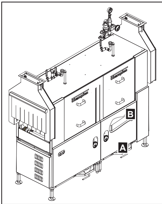
Fig. 9 - Connect Wires Between TLS and the Terminal Block in the Control Cabinet.
