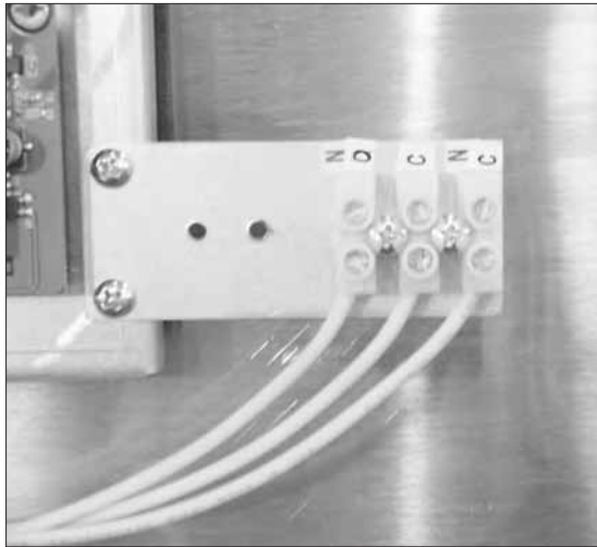
The Low temperature interlock block is located on the right-side of the booster cabinet interior.
