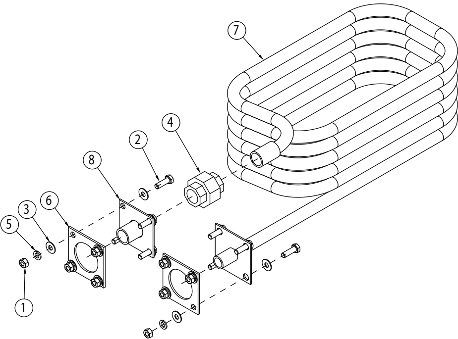
STEAM SUPPLY AND CONDENSATE PIPING SHOWN WITH 1200 THRUSH BOOSTER
