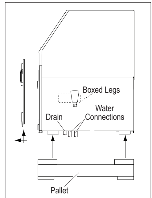
Glasswasher plumbing connections extend below the pallet.
