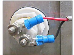
Fig. 32- Tank sensor
