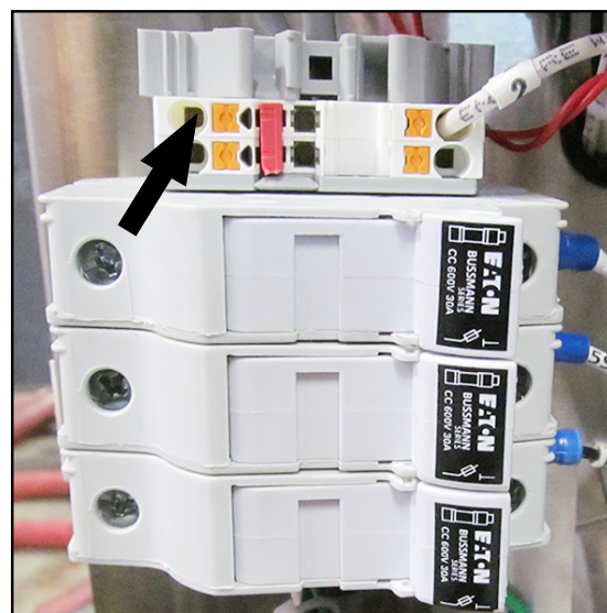
Fig. 22- Rinse aid signal connection
