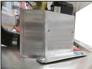
Fig. 2 - Mounting bracket
