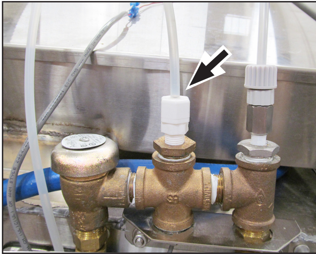
Fig. 20 - Rinse aid injection point
