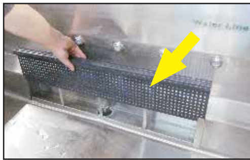
Fig. 12 - Install wash tank pump screen.
