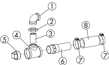
Recirculating Pump Trough Connection Kit: P/N 407365
