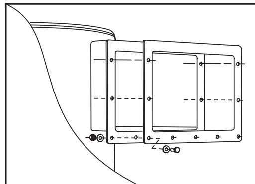
Rubber gasket for a trough connection is supplied with the pulper.
