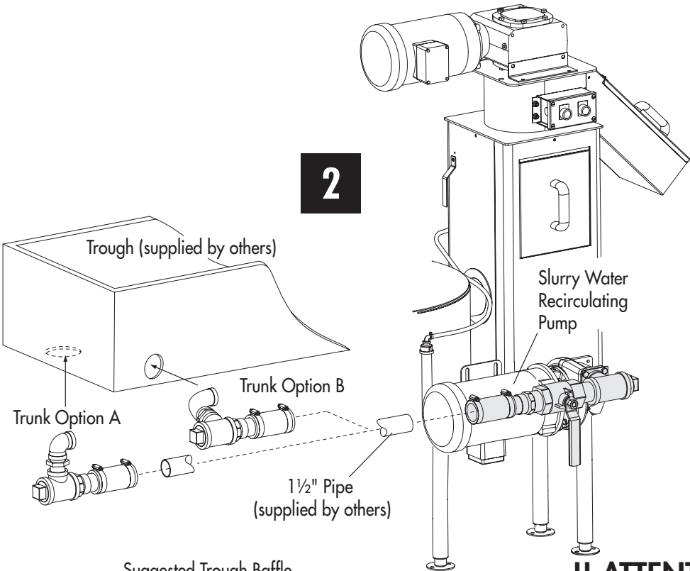
Recirculating Pump Trough Connection Kit: P/N 407365
