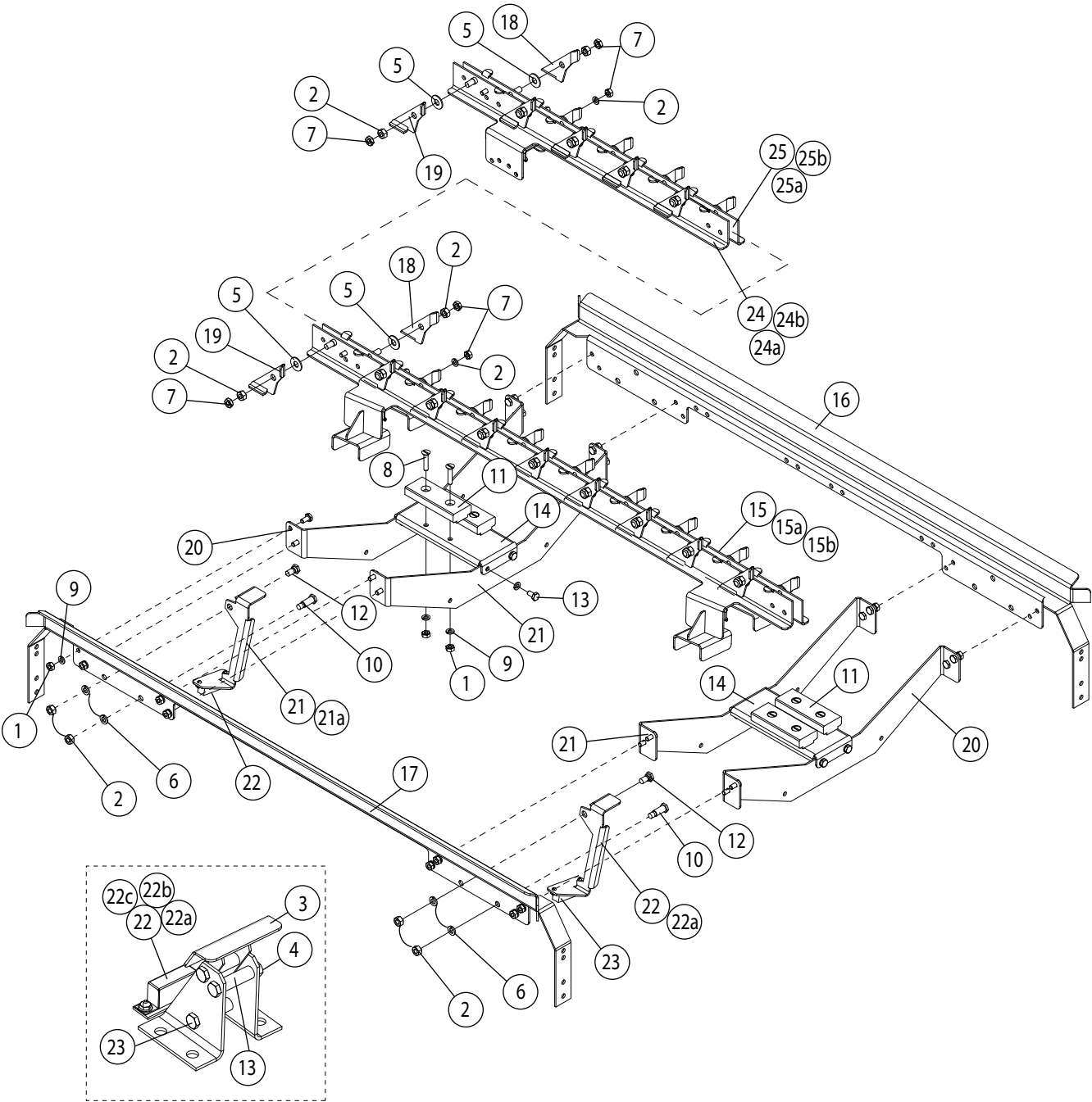
VHR Idle Pump Assembly
