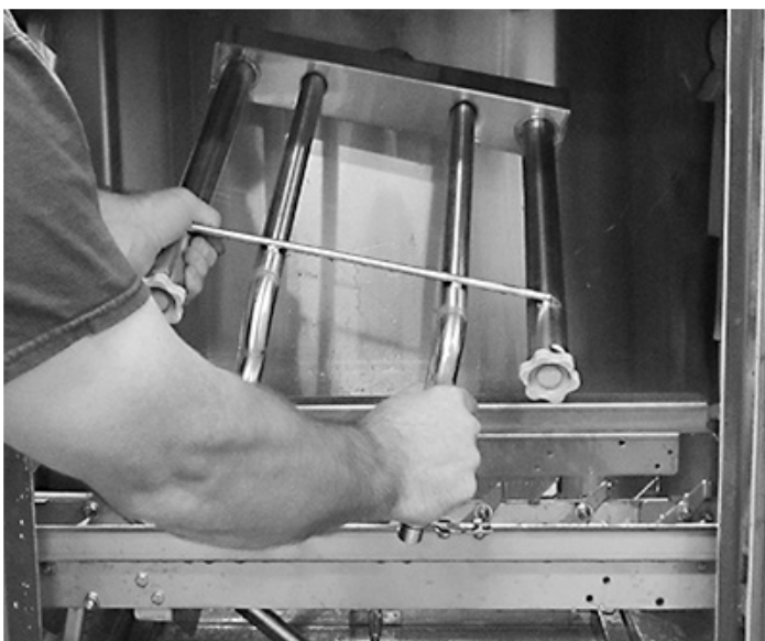
Fig.9 - 36" Prewash Tank
