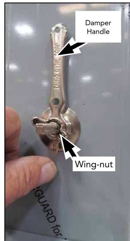
Fig. 8a- Duct.
