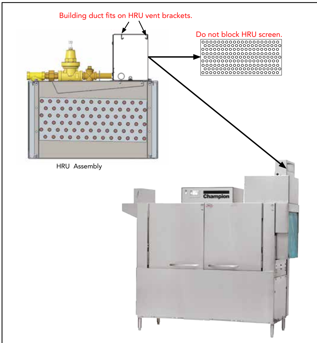
Fig. 9 - Do not block screen when installing building venting.
