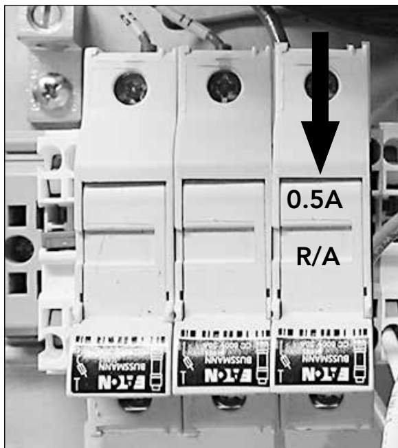
Fig. 11 Rinse Aid Connection
