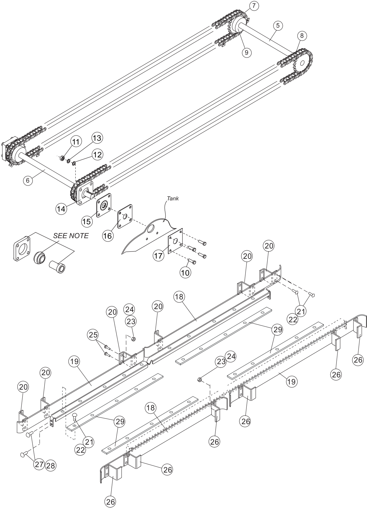
Figure 6.5a - Conveyor shafts, chains, bearings and guides (From S/N J1050 and Above)
