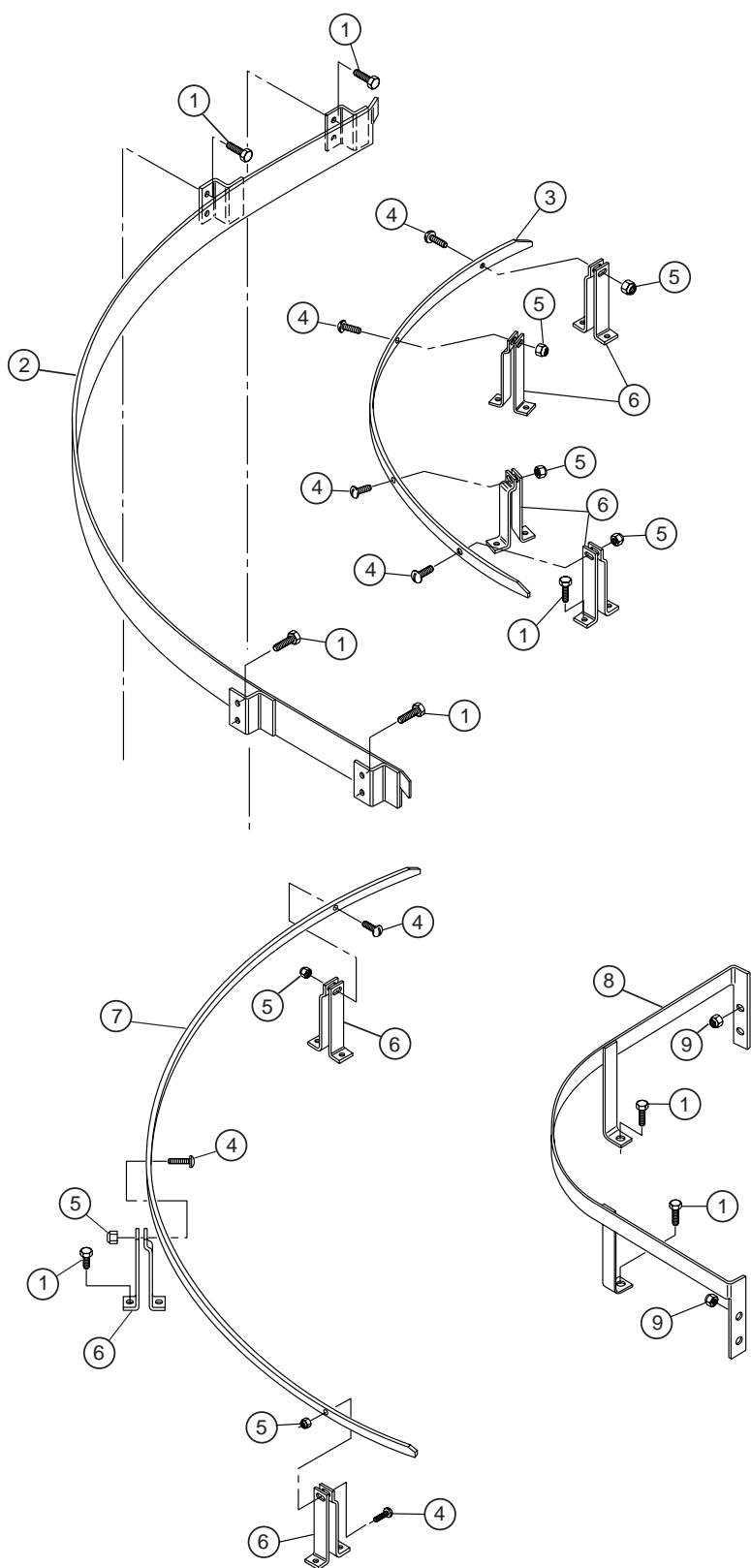
Figure 6.19- MRAN 90° Guides
