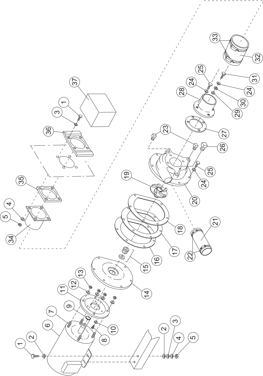
Figure 6.13 - Pump assembly
