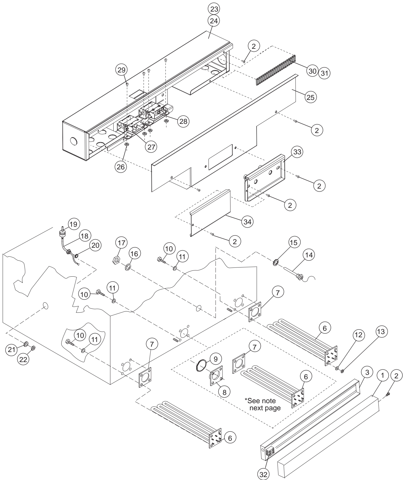
Figure 6.9a - Electric Tank Heat (For machines beginning with S/N J1050 through J1871) Left-Right Installation Shown
