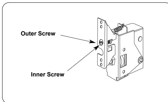
Figure 19. Thermostat Adjustment
