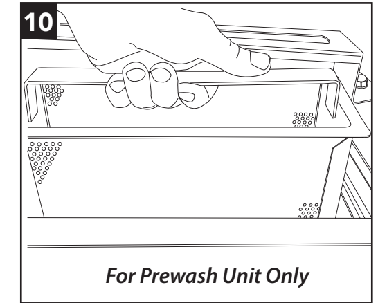
10 Remove the refuse basket and back-flush in a sink. Do not strike the basket on hard surfaces.
