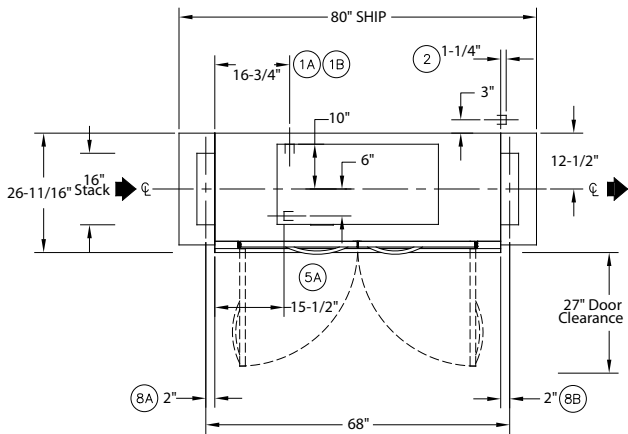
Plan View Left to Right
